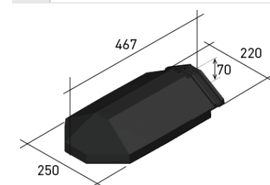
14 ORTGANGZIEGEL LINKS
