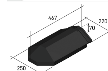
14 ORTGANGZIEGEL LINKS
