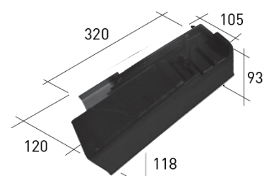
15 HALBER ZIEGEL LINKS
